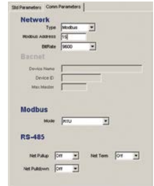
Figure 4: Comm parameters—modbus
